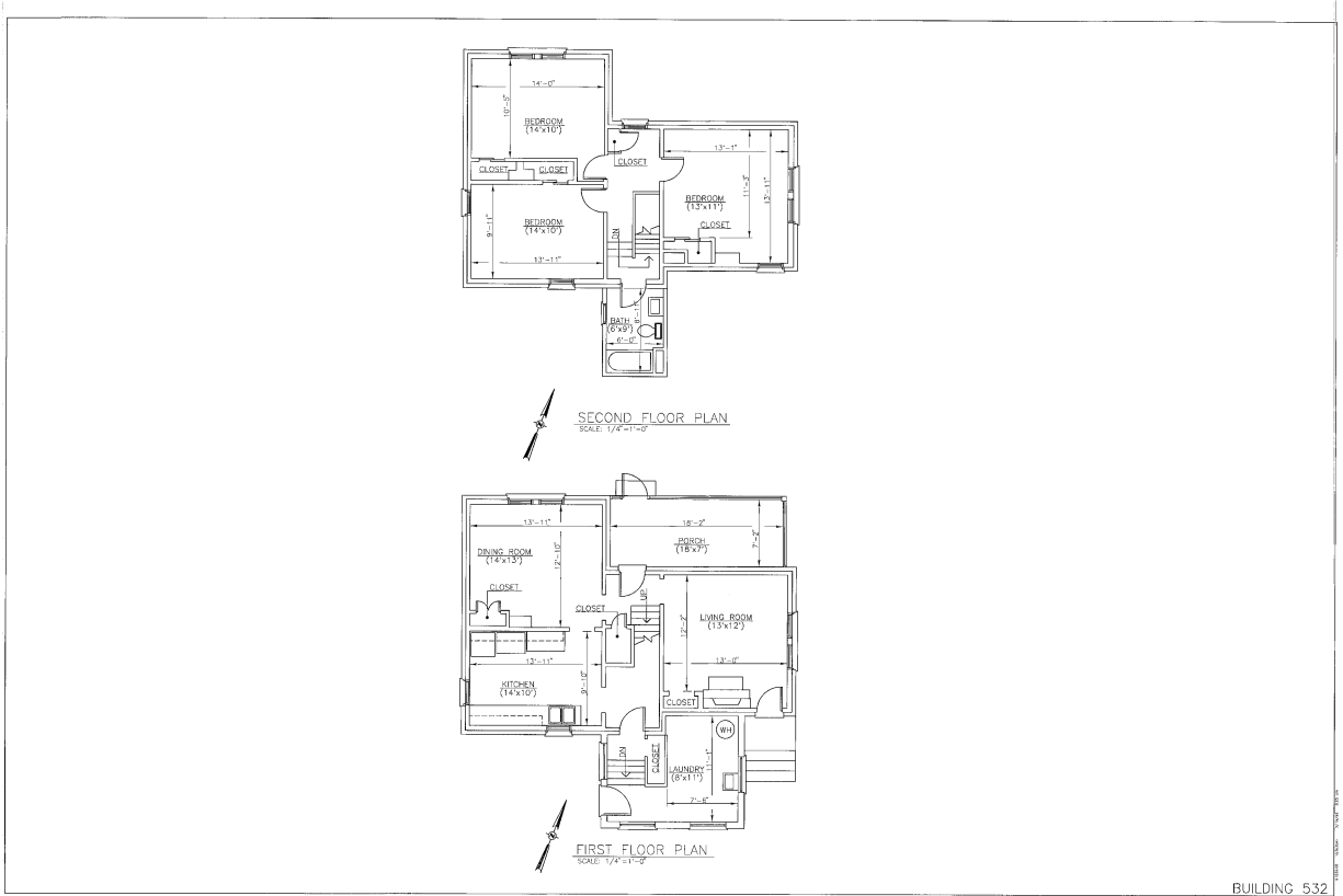
Figure 1: Building 532 1 st & 2 nd floor plan
